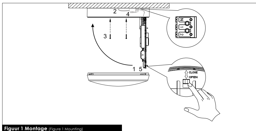
Figuur 1 Montage (Figure 1 Mounting)
