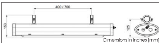
Ceiling Mount
