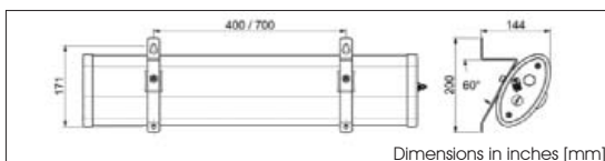
Wall Mount Bracket 60°
